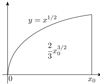
Figure 31. Newton's calculus
