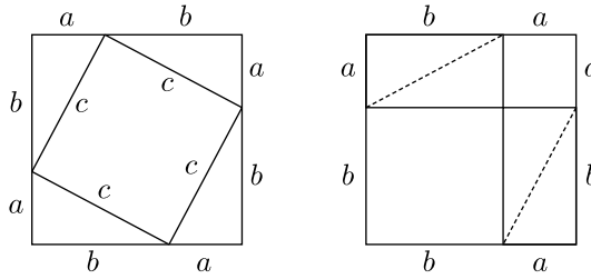
Figure 6. Pythagoras' Theorem
