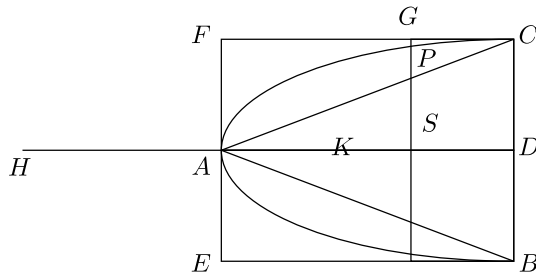
Figure 25. Paraboloid of revolution and cone
